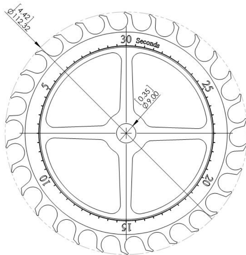
Escapement wheel (38) 1X
