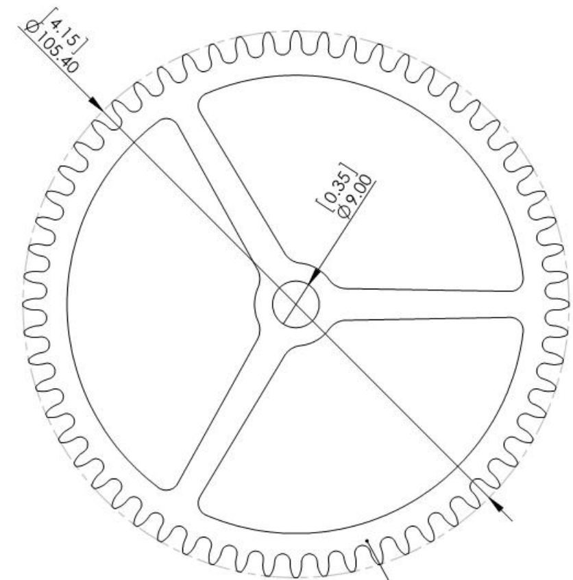
Gear 60 Teeth (49) 4X
