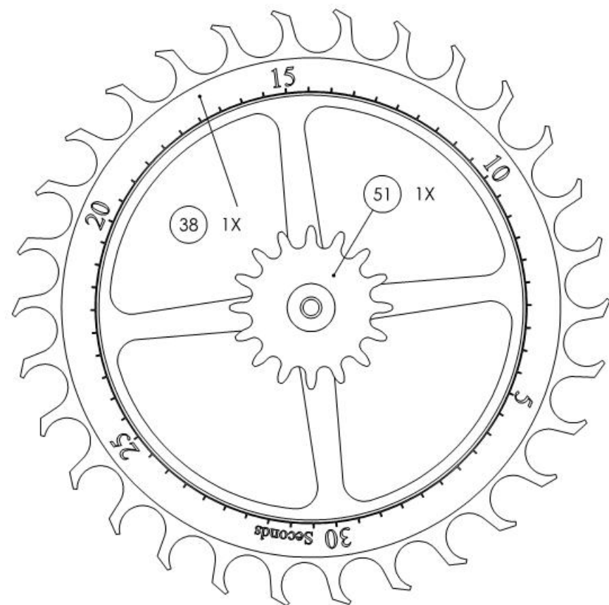
Escape wheel Sub Assembly
