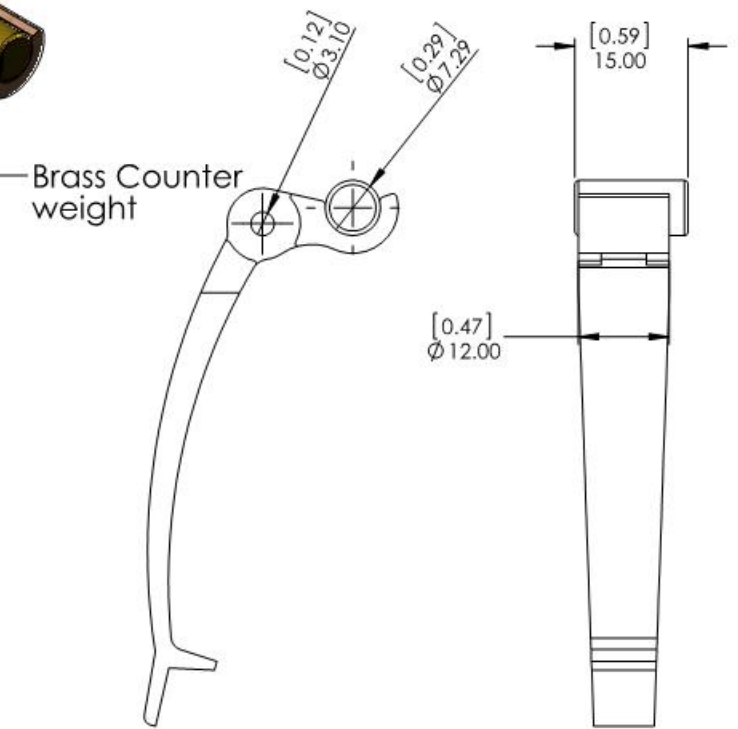
1X (69) Grasshopper RH Arm Scale 1:1
