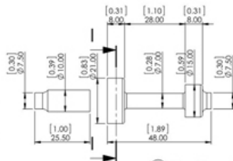
1X 12 Gear Sleeve for 48T Scale 1:1
