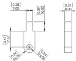
1X (38) Verge Support Scale 1:1
