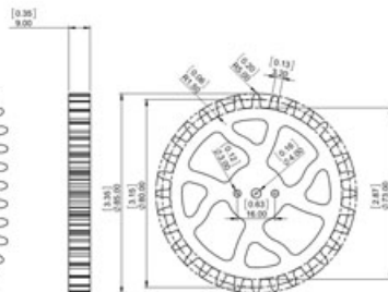
1X 28 Winder Gear 32 Teeth Scale 1:1 Wood
