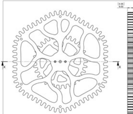
Drive Train 2
