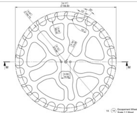
1X 14 Escape Wheel Scale 1:1 Wood
