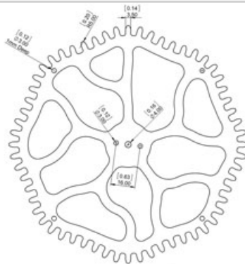
1X 16 Gear 50 Teeth 8 repeats Scale 1:1 Wood
