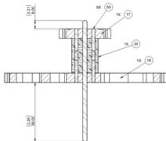
SECTION W-W SCALE 1:1
