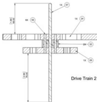
Drive Train 2
