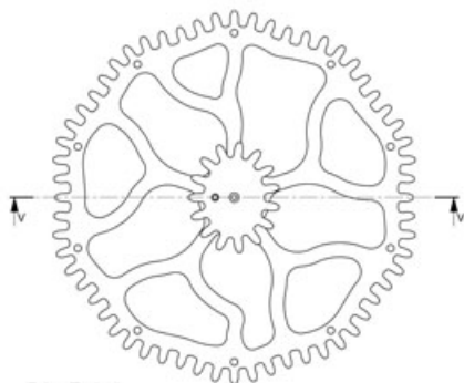
Drive Train 4
