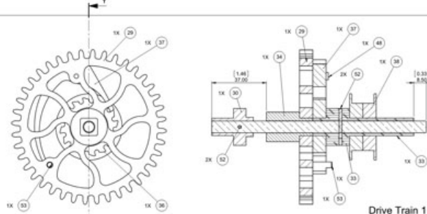
Drive Train 1
